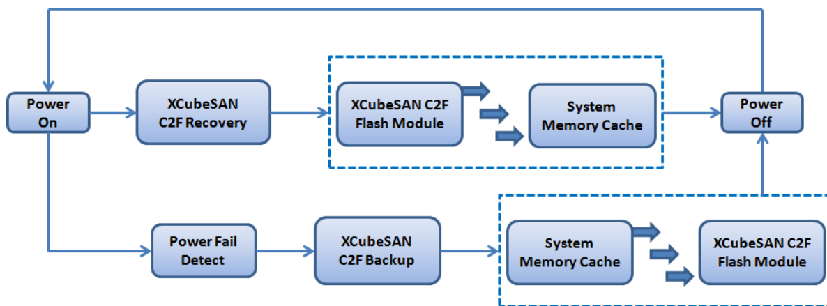
Figure 2-15 Cache-to-Flash Workflow
